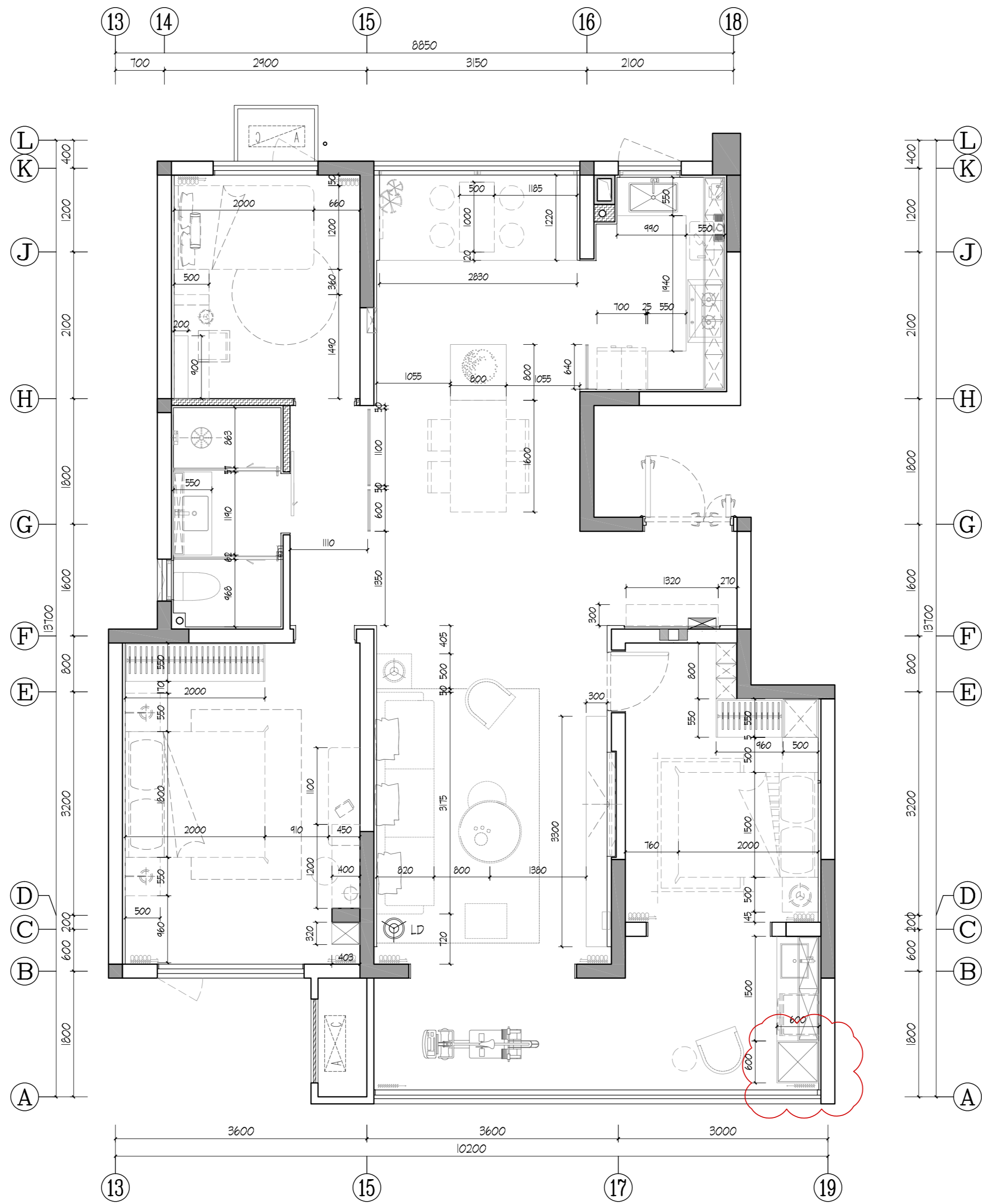
01 FURNITURE DIMENSION PLAN 家具定位图 SCALE 1: 50
