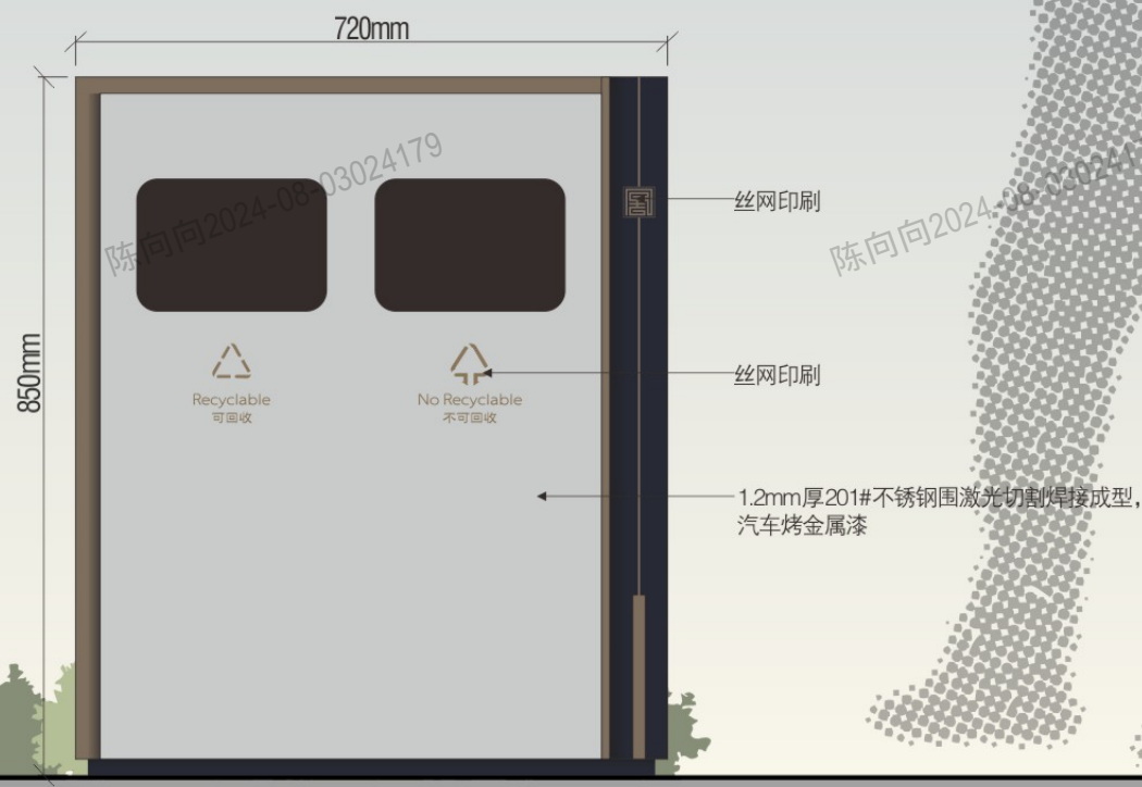
1 立面-Elevation 1:10
