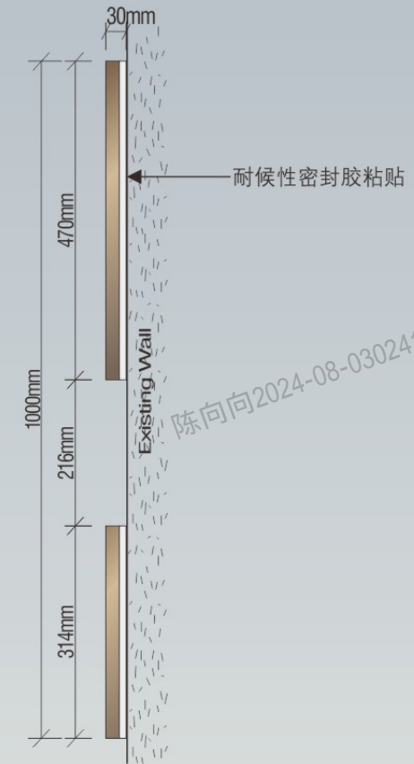
2 侧立面-Side Elevation 1:10
