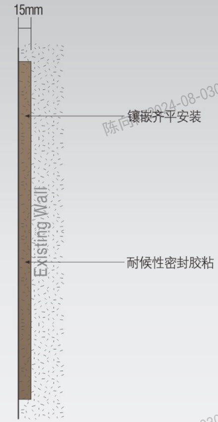
2 侧立面-Side Elevation 1:10
