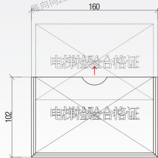
3 尺寸详图- Section Detail 1:5
