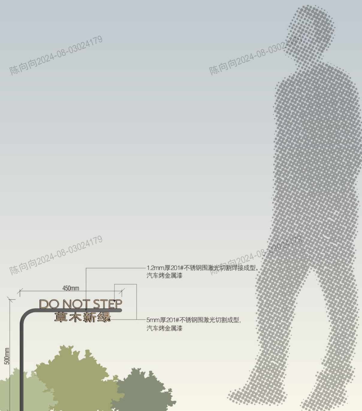
1 正视图-Elevation 1:10
